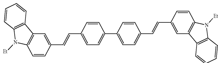
BCzVBi
