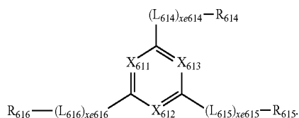
Chemical Formula 602
